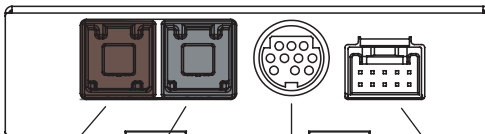
Brown USB interface connector Grey USB interface connector Interface connector for SiriusXM SXV300 Tuner Power connector
